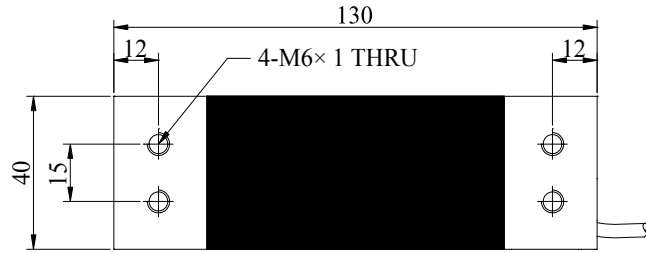
俯視 (Top View)
