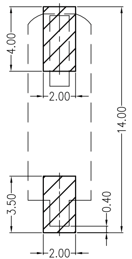
Board Layout
