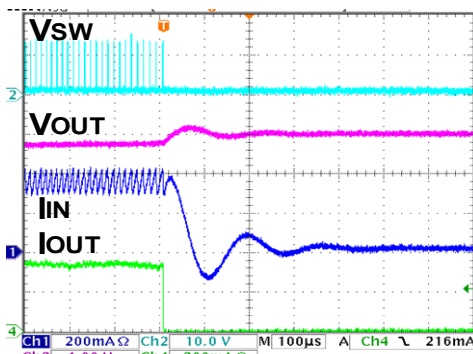
Figure 61. Open-circuit protection
