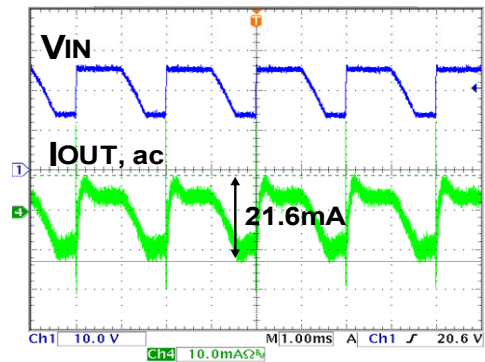
Fig49. L1=68\mu H
