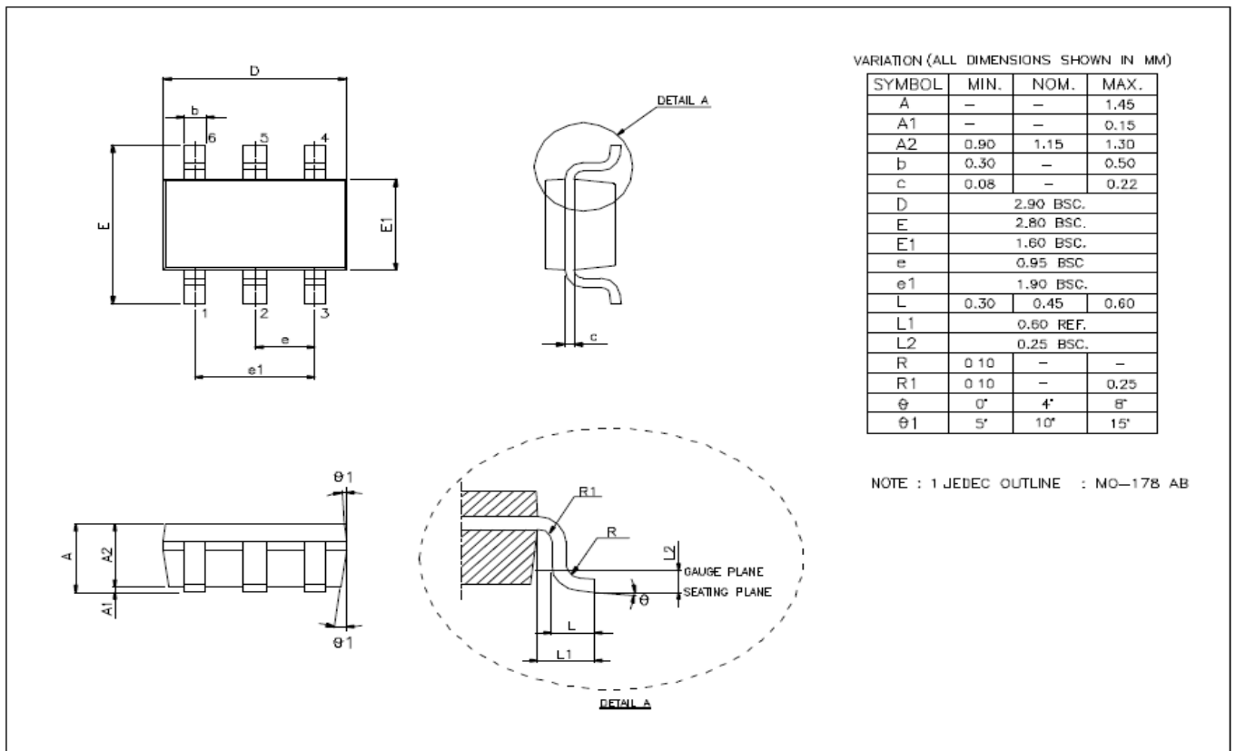
MBI6652GST Outline Drawing
