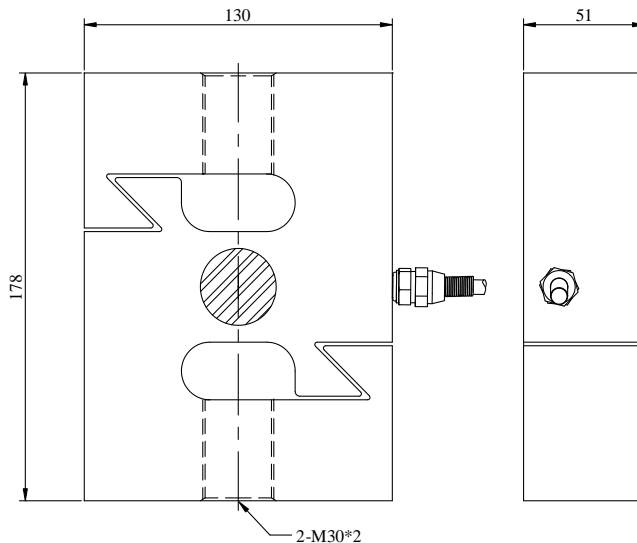
主視 (Front View) 右視 (Right View)
