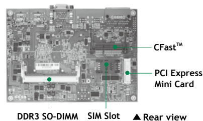
DDR3 SO-DIMM SIM Slot ▲ Rear view
