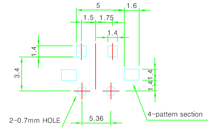
PCB PATTERN
