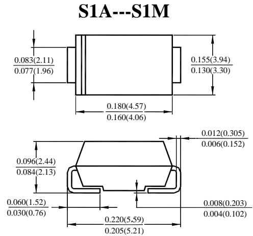
Dimensions in inches and (millimeters) DO-214AA (SMB)
