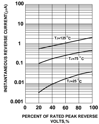
FIG.4-TYPICAL REVERSE CHARACTERISTICS
