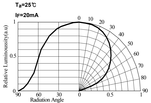
Radiation Diagram
