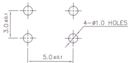
PCB DIMENSION
