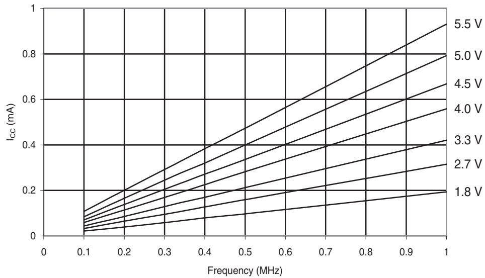
Figure 30-142.ATmega88PA: Active Supply Current vs. Low Frequency (0.1-1.0MHz)
