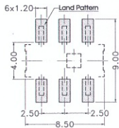
PIERCING PLAN
