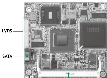
DDR2 SO-DIMM
