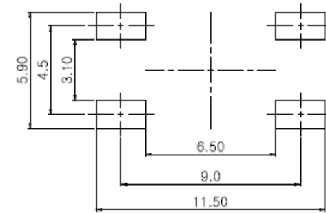
PCB PATTERN DIMENSIONS
