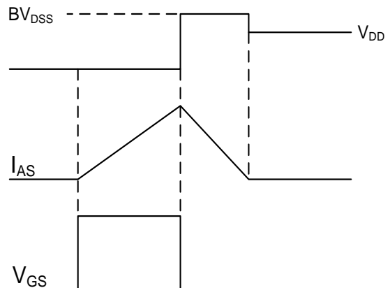
Fig.12 EAS Waveform
