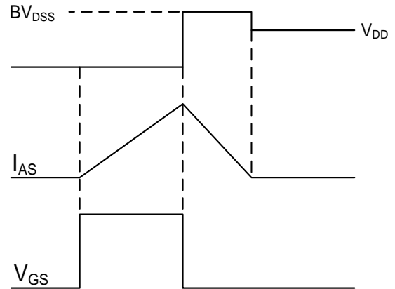
Fig.10 EAS Waveform
