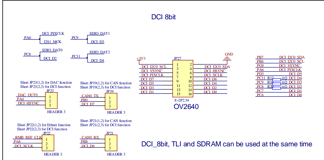
Figure 4-16 Schematic diagram of DCI function
