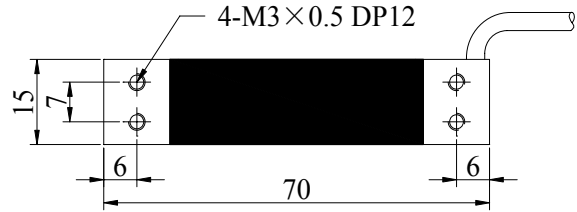
俯视(Top View)
