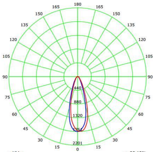
Luminous Intensity Distribution Curve(cd/klm)
