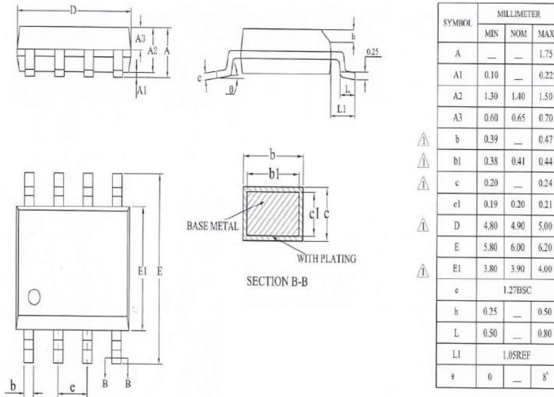
Figure 21 - 1 SOP8 package size
