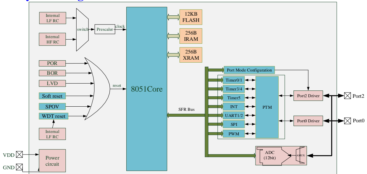
Figure 1-1 System diagram
