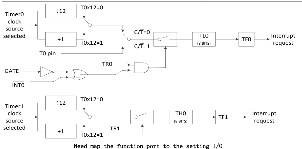
Figure 9 - 4 Timer0 3 function block diagram
