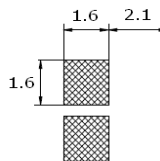
4520 PAD LAYOUT
