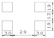
7060 PAD LAYOUT
