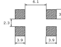
1211 PAD LAYOUT
