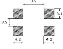
1513 PAD LAYOUT
