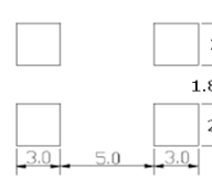
9070 PAD LAYOUT
