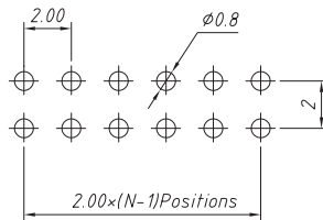
Recommended P.C.B Hole Layout
