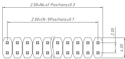
Recommended P.C.B Hole Layout
