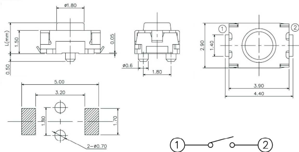
Mounting Holes
