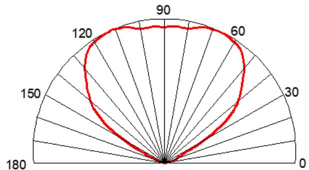
Fig.8 Radiation pattern@30mA
