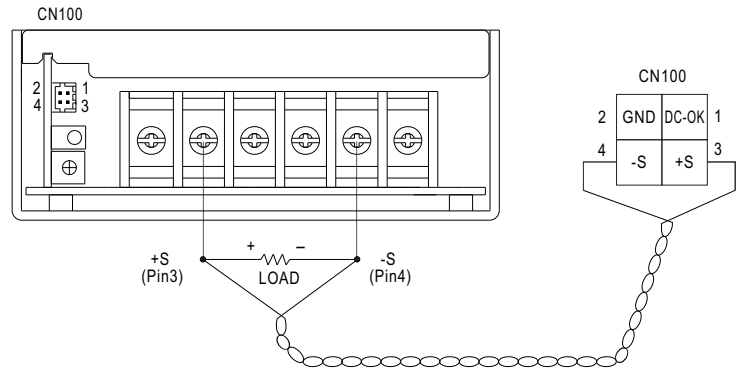
Fig 1.1 Sense lines should be twisted in pairs
