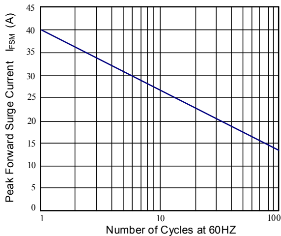
Figure 6: Maximum Non-Repetitive Forward Surge Current Only Unidirectional
