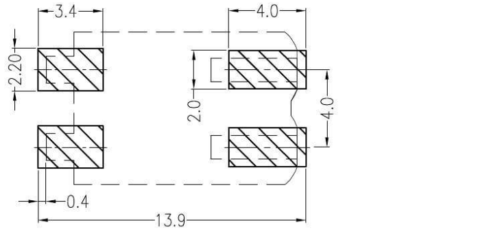
Board Layout
