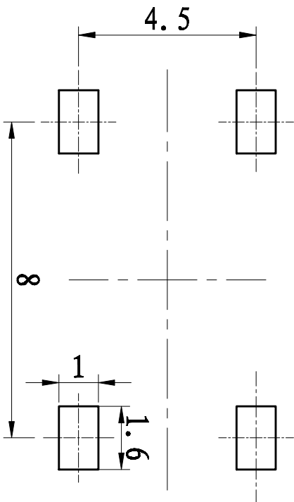
Suggested P.C.B Layout
