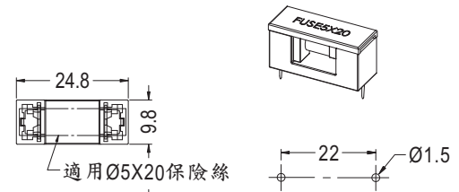
MOUNTING HOLES
