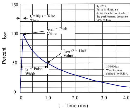
Figure 3: Pulse Waveform
