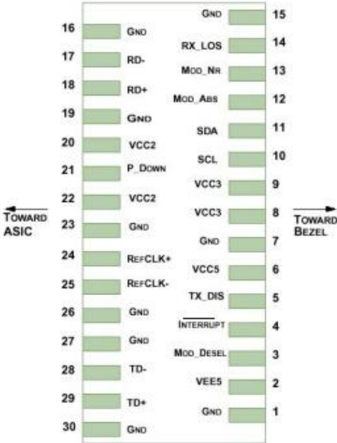
Pin-out of Connector Block on Host Board
