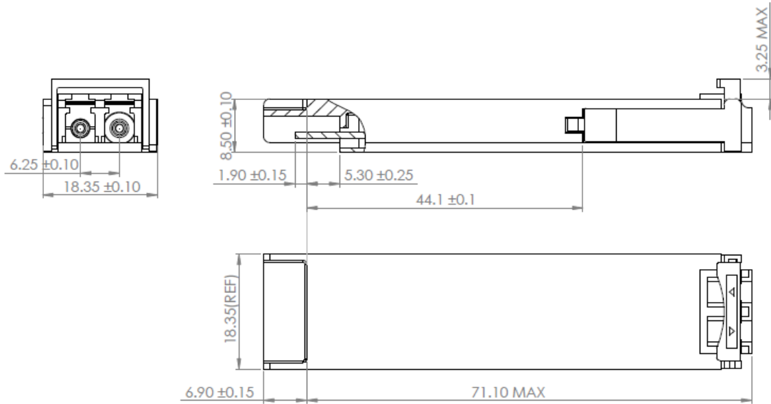
SFP-XCxxHM0xDL40
